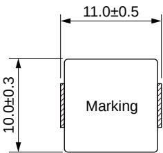
Dimensions: [mm]
