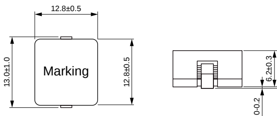
Dimensions: [mm]
